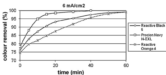
Fig. 5. Evolution of colour removal for Reactive Orange 4, Reactive Black 5 and Procion Navy H-EXL after electrochemical treatment (6 \text{mA/cm}^2 ) plus UV light irradiation of effluents containing 0.5 \text{g L}^{-1} NaCl.
