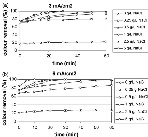
Fig. 3. Influence of different NaCl concentrations on colour removal of Reactive Orange 4 ( 0.1 \text{ g L}^{-1} ) due to UV light exposure ( 254 \text{ nm} , 6 \text{ W} ) after electrochemical treatment ( 20 \text{ L h}^{-1} ). Current density: (a) 3 \text{ mA/cm}^2 and (b) 6 \text{ mA/cm}^2 .
