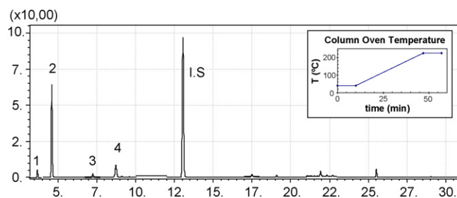
Fig. 4. Chromatogram of Reactive Orange 4 treated at 3 \text{ mA}/\text{cm}^2 and containing 0.5 \text{ g L}^{-1} of NaCl. (1) Dichloromethane, (2) chloroform, (3) trichloroethylene and (4) bromodichloromethane. I.S. is the internal standard, p-bromofluorobenzene.
